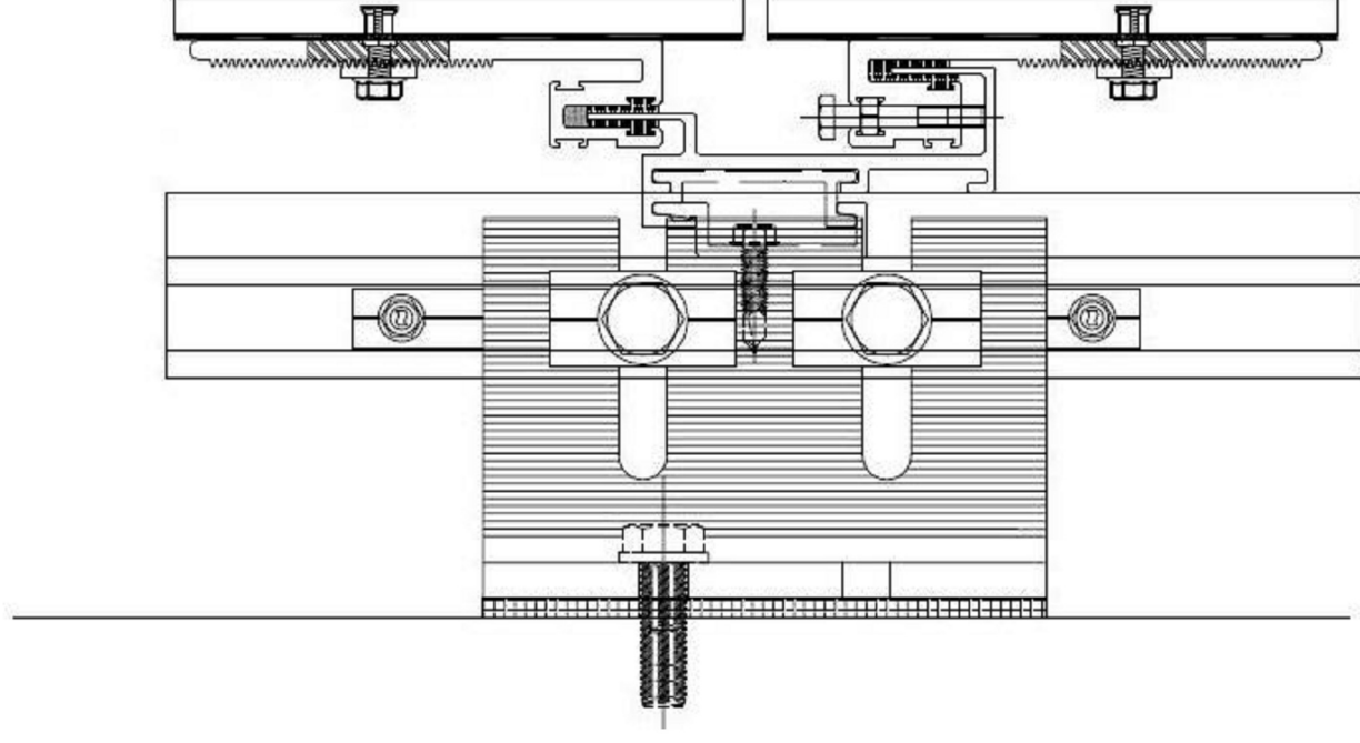
1cm CFR Natural Stone Cladding on eclair E1V system
