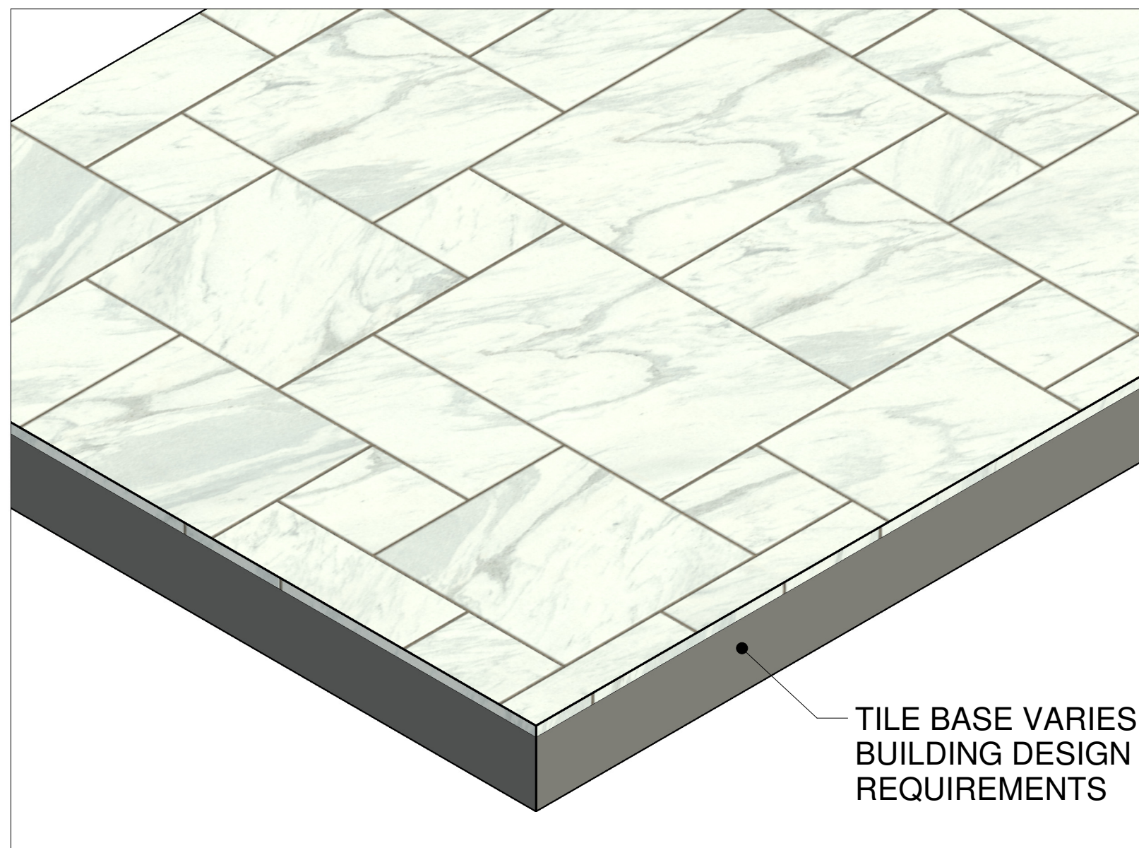
POLYCOR STONE FLOOR TILE - 1 1/4" THICK
