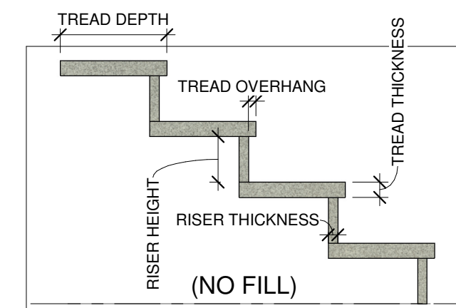
2 TO 6 STEP ASSEMBLY CUSTOMIZABLE STEP PROPERTIES INCLUDES STEP WIDTH
