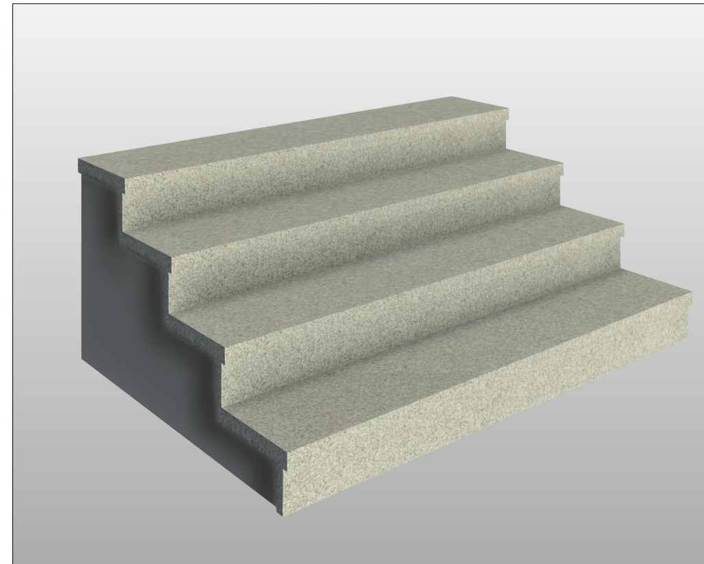
TREAD - 72" x 14" x 2" RISER - 72" x 5" x 1 1/4" INDIVIDUALLY PLACED BARRE GRAY™ GRANITE
